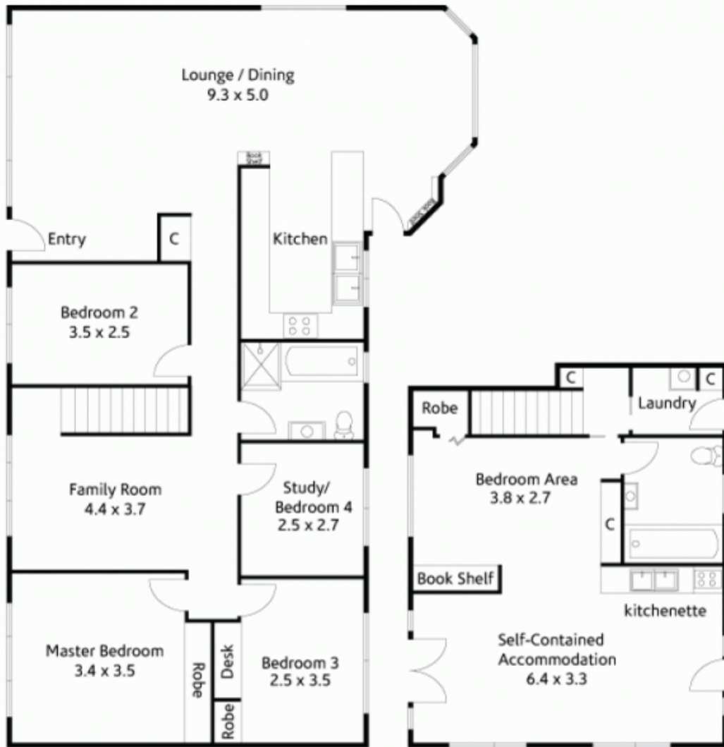
Ground Level
