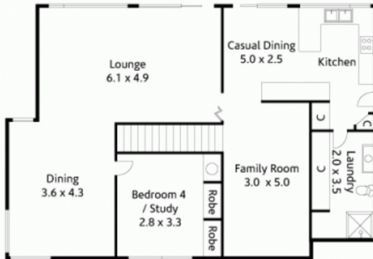
Lower Level
