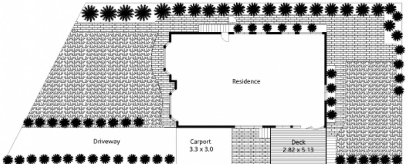
Site Plan
