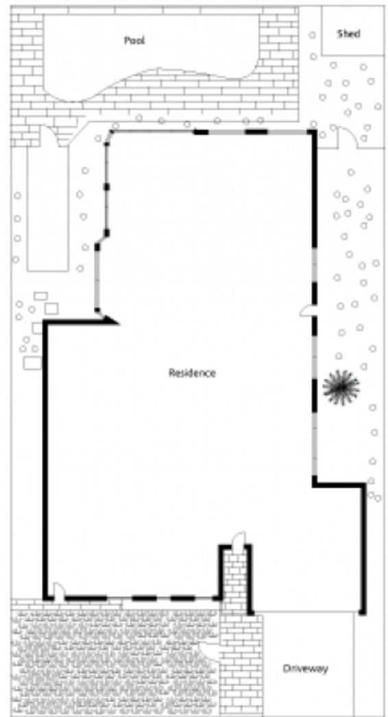
Site plan
