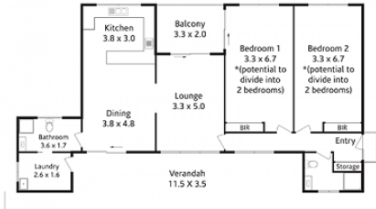
Upper Ground Floor
